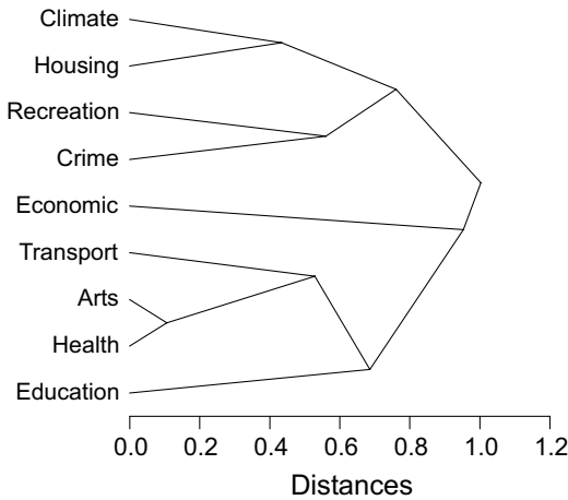
Figure 7.35 Cluster tree
