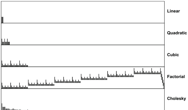
Figure 16.17 Complexity graphs
