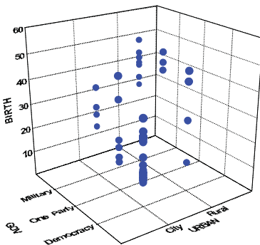
Figure 8.2 3D points on categorical (left) and continuous (right) domains
