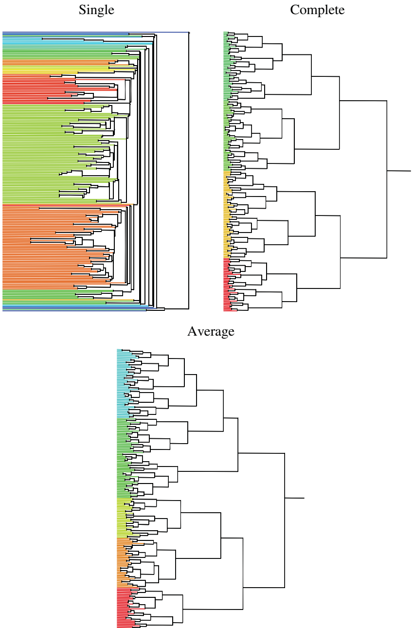
Figure 13.26 Cluster trees on anemone data
