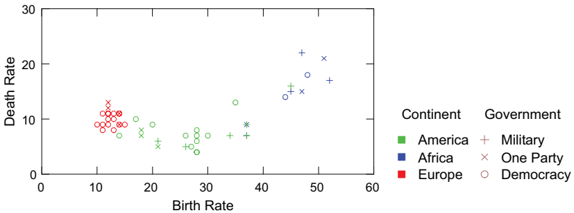
Figure 12.1 Double legend
