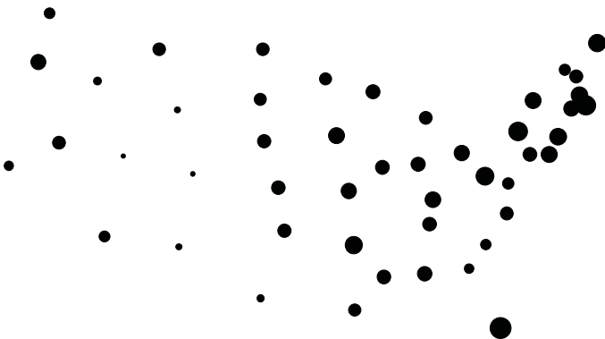
Figure 13.20 US cancer rates
