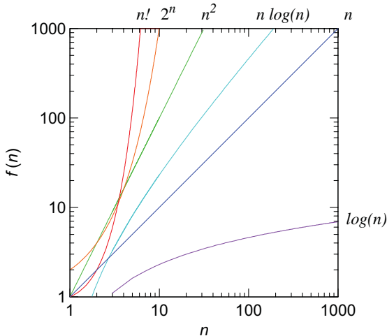
Figure 16.16 Complexity functions
