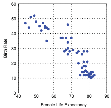
Figure 8.1 A point cloud on categorical (left) and continuous (right) domains
