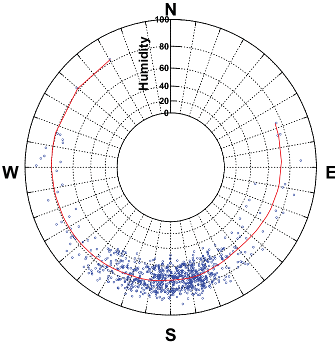
Figure 9.17 Conformal mapping
