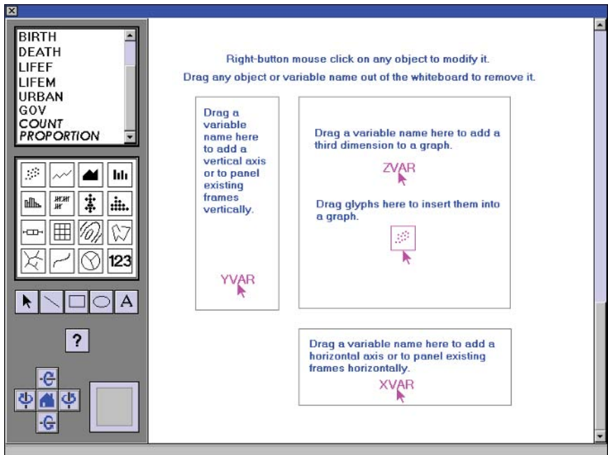
Figure 17.5 Graphboard help (?)
