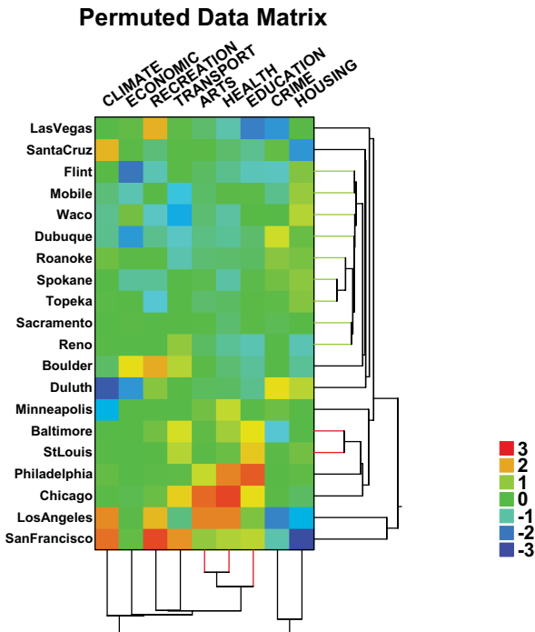
Figure 18.2 Permuted tiling
