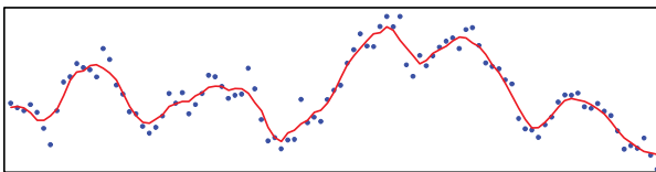
Figure 14.21 Moving average of random walk
