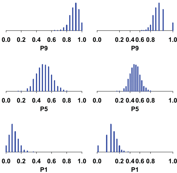
Figure 6.11 Proportion of heads in 25 tosses for \pi = .1, .5, .9 (1,000 samples)
