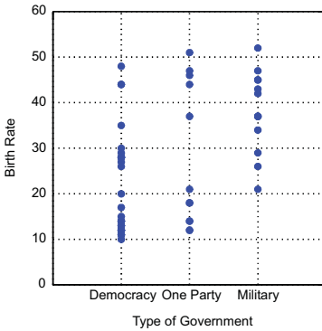
Figure 8.1 A point cloud on categorical (left) and continuous (right) domains
