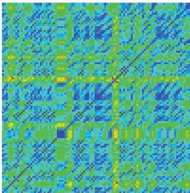
Figure 14.14 Recurrence plots
