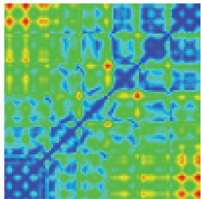
Figure 14.14 Recurrence plots
