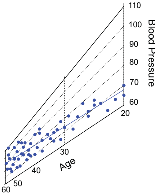
Figure 9.15 Projection
