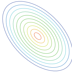
Figure 13.16 Mahalanobis anisotropic isodistance contours
