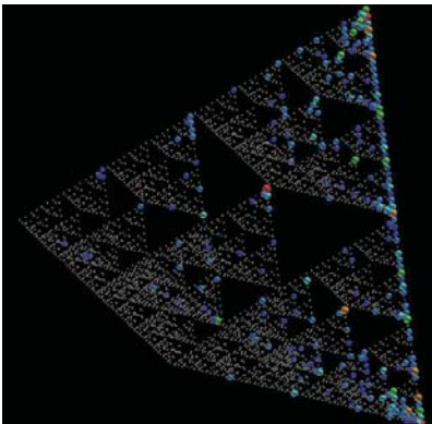
Figure 13.24 Carr Sierpinski Gasket (courtesy Dan Carr)
