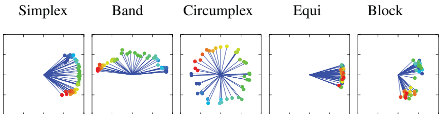
Figure 16.27 Two-dimensional factor solutions
