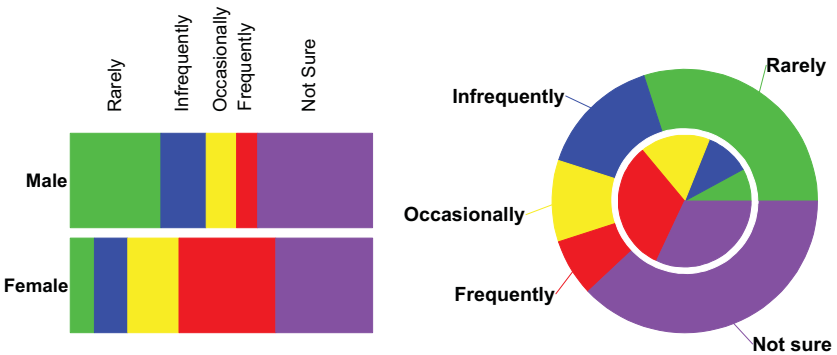
Figure 9.26 Polar divided bar of ACLS data
