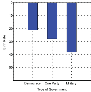
Figure 9.4 Vertical reflection
