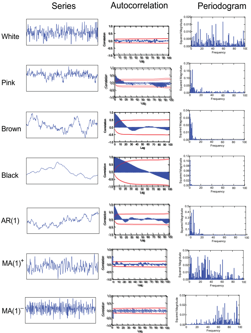
Figure 14.6 Stochastic series
