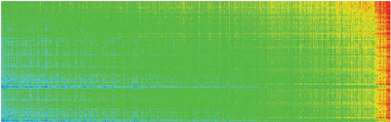
Figure 7.25 Microarray plot
