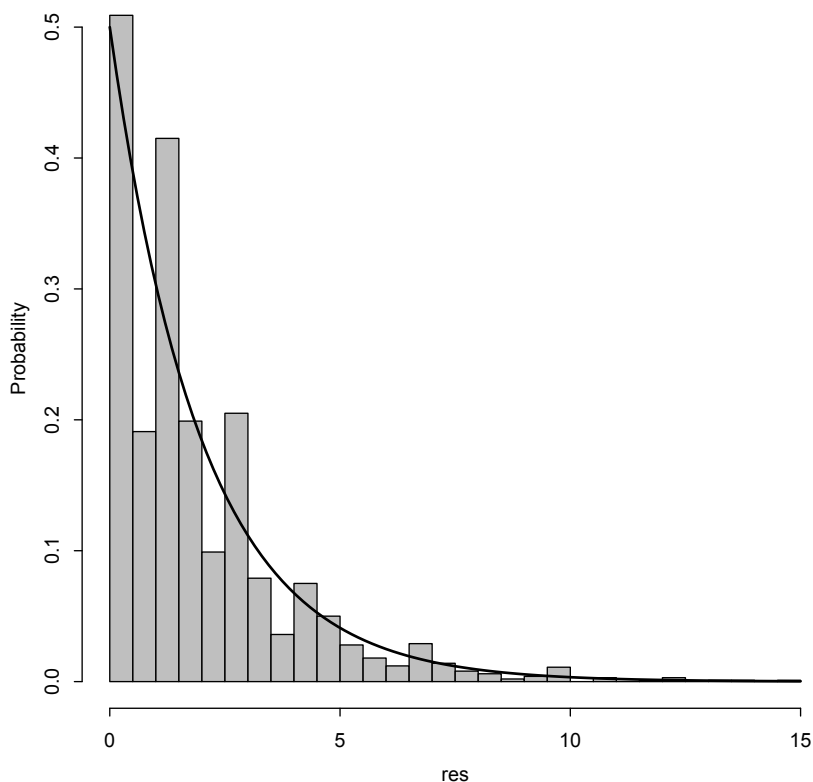
Figure 10.1: Simulation of \chi^2 -statistic with n = 20 and probabilities 3/12 , 4/12 , and 5/12 . The chi-squared density with 2 = k - 1 degrees of freedom is added.
