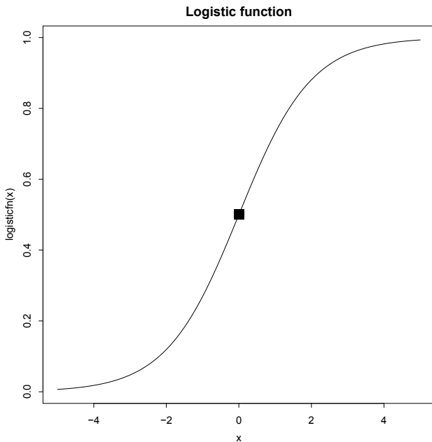
Figure 13.1: Graph of logistic function, m(x) = e^x / (1 + e^x) . The inflection point is marked with a square.
