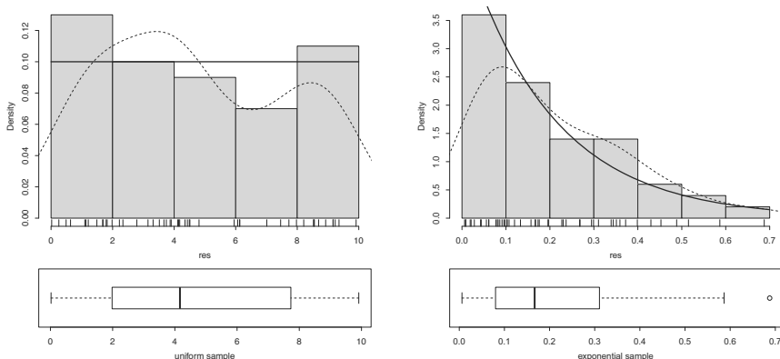
Figure 6.7: Histogram and boxplot of 50 samples from the Uniform(0,10) distribution and the Exponential(1/5) distribution. Both empirical densities and population densities are drawn.
