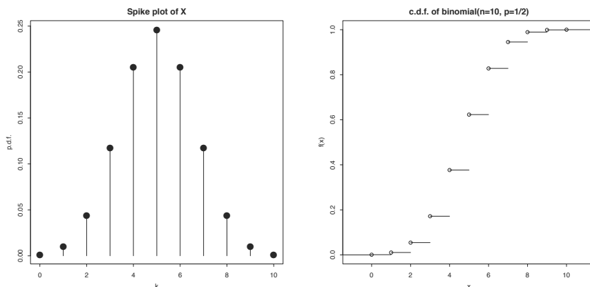
Figure 6.5: Spike plot of Binomial(10,1/2) distribution, and plot of its cumulative distribution function.
