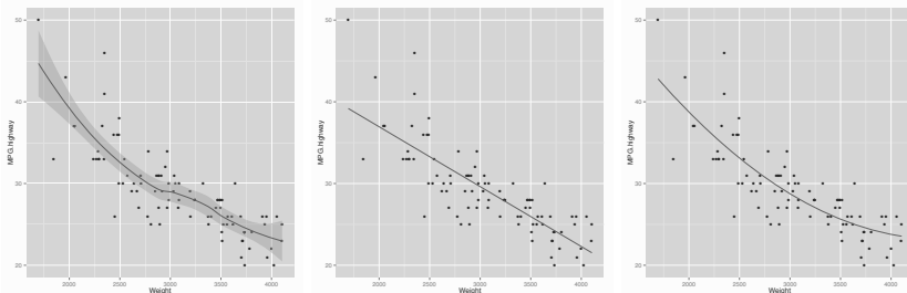
Figure 5.13: For the same scatterplot, three different trend lines are added. The first the default computed by loess and showing an estimated confidence band, the second a linear regression line, and the third a quadratic polynomial fit.
