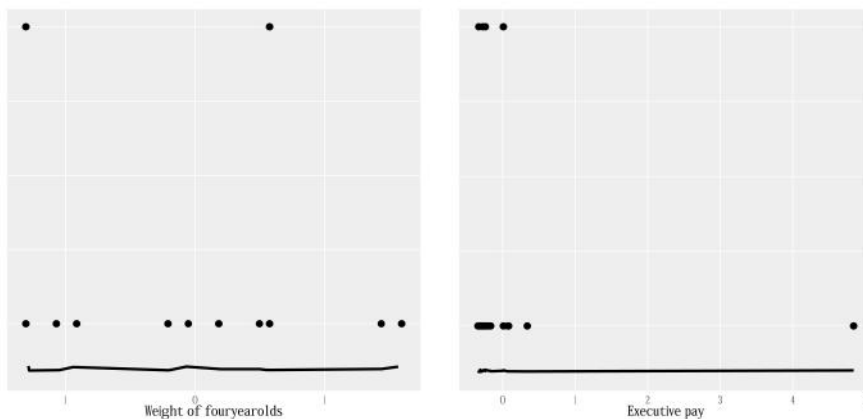
Figure 2.3: Plot of absolute z-scores for the wts data set and a subset of the exec.pay data set. There are no values larger than 2 in the wts data set, in agreement with the rule of thumb for bell-shaped data. For the executive pay data, we see a z-score nearly as large as 5, virtually impossible for bell-shaped data.
