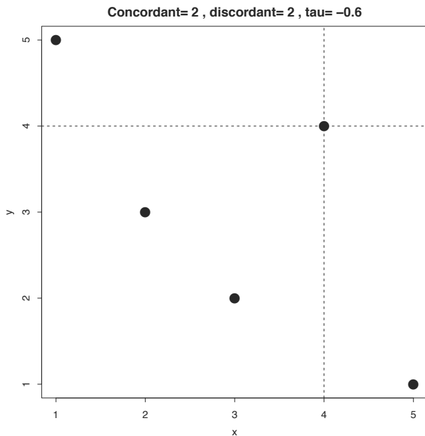
Figure 3.23: Scatter Plot of ranked data with focus on one point. For this value, there are 2 points in the third quadrant (concordant) and one each in the second and fourth quadrant (discordant), a difference of 0. Moving the crosshairs over all n points and adding the differences gives the numerator in the Kendall correlation.
