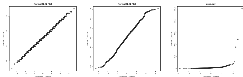
Figure 2.10: Three quantile-normal plots produced by qqnorm . The leftmost graphic shows data on finger lengths of several prisoners from the finger variable in the Macdonnell ( HistData ) data set. It shows data more or less on a straight line, indicating a normal distribution. The grouping is due to the data being discretized. The second graphic uses data on the height of children in Galton's classic study of heights. This data has slight bends on the edges, like an "S". This being due to the tails being slightly less long than the normal. The final data shows what a decidedly non-normal distribution appears like in this graphic. The executive pay data is used which is skewed right and long tailed. Such data shows a clear curve.
