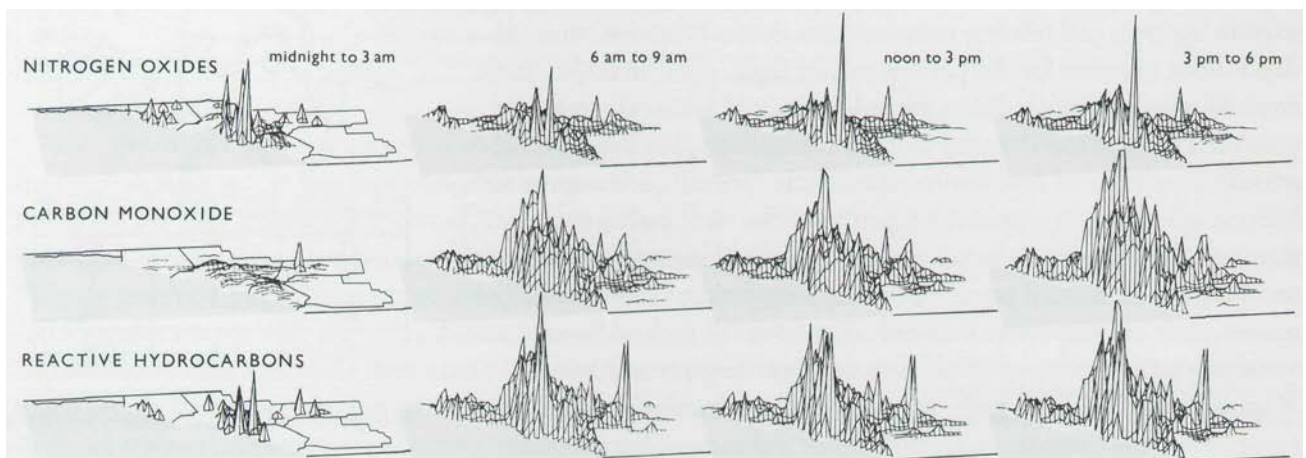
Redrawn. See G. J. McRae, W. R. Goodin, and J. H. Seinfeld, "Development of a Second-Generation Mathematical Model for Urban Air Pollution. I. Model Formulation," Atmospheric Environment , 16 (1982), 679-696.
