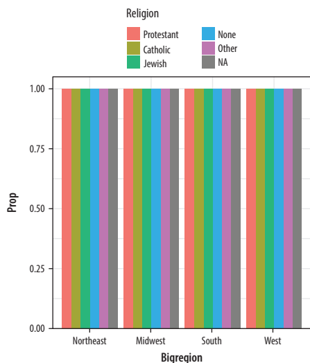
Figure 4.12: A first go at a dodged bar chart with proportional bars.
