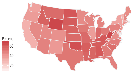
Figure 7.8: Two versions of percent Trump by state.
