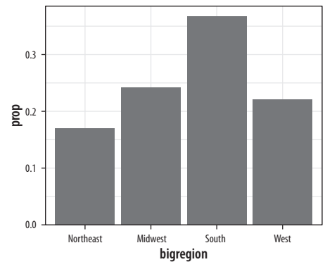
Figure 4.8: A bar chart with correct proportions.
