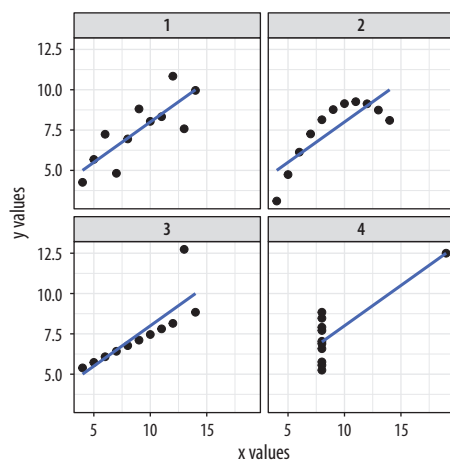
Figure 1.1: Plots of Anscombe's quartet.
